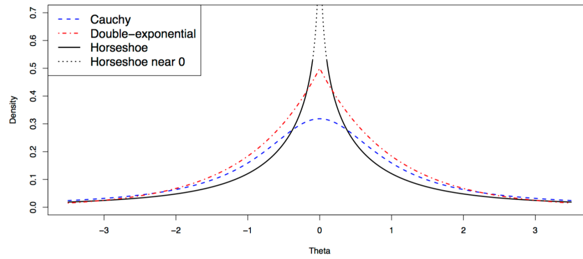
Tails of different priors
